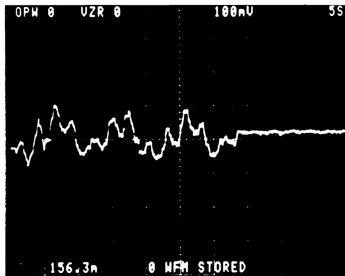
Fig. 6. Transition from uncontrolled spindle runout to controlled spindle runout. Vertical scale = 1.3 \mu\text{m} ( 55 \mu\text{in.} ) / division; horizontal scale = 180^\circ rotation / division.
