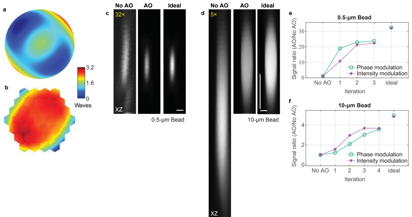
Extended Data Fig. 3 | Correcting artificial aberrations for 2P microscopy using phase versus intensity modulation and signal from fluorescent features of different sizes. a,b , Artificial aberration introduced with the SLM and corrective wavefront on the DM, respectively. c,d , Axial images of 0.5- \mu m- and 10- \mu m-diameter fluorescent beads, respectively, without AO, with AO (phase modulation), and under ideal aberration-free conditions (without artificial aberrations applied to the SLM). Digital gains were applied to No AO images to increase visibility. Post-objective power: 6 and 2.3 mW, respectively. e,f , 2P signal versus iteration number for 0.5- \mu m- and 10- \mu m-diameter beads, respectively, using phase and intensity modulation. Scale bars: 1 \mu m in c and 5 \mu m in d . Microscope objective used: NA 0.8 16 \times . n=1 bead in c and d , respectively.
