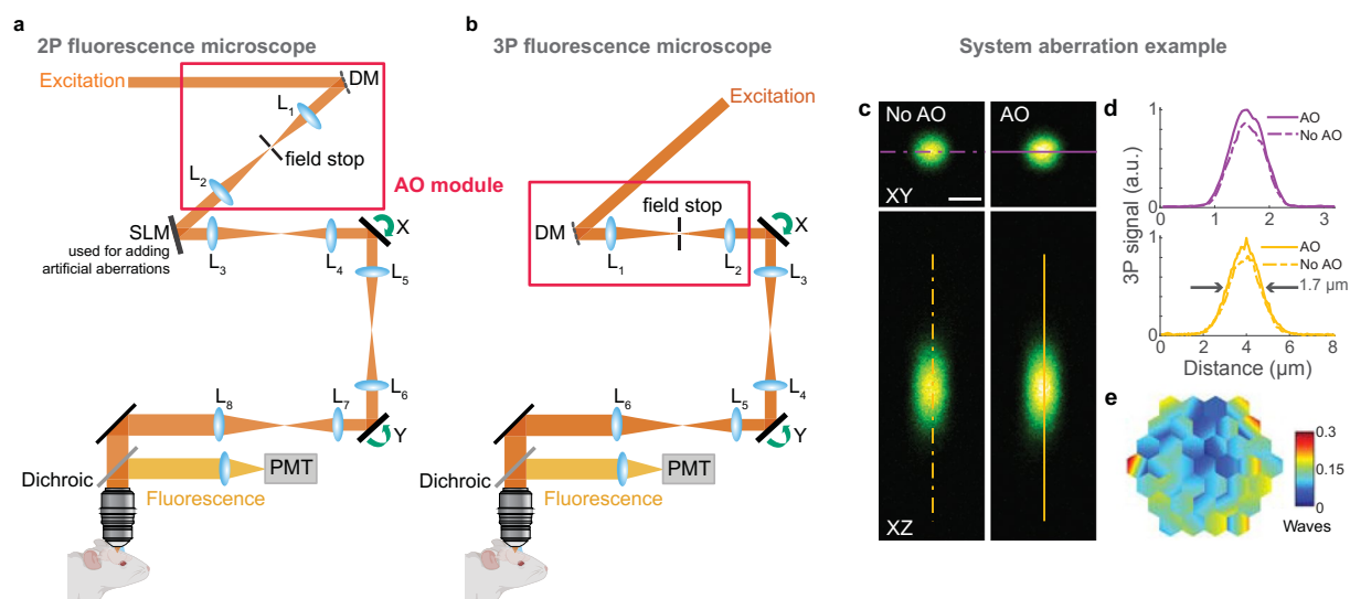
Extended Data Fig. 2 | Schematics of AO 2P and 3P fluorescence microscopes, and example system correction. a,b , Components of AO 2P and 3P fluorescence microscopes, respectively. DM, deformable mirror; SLM, spatial light modulator (used to introduce artificial aberration); L, lenses; X and Y, galvanometers; PMT, photomultiplier tube. c , Lateral and axial 3P images of a 1- \mu\text{m} -diameter red fluorescent bead, under 1300 nm excitation, taken without and with AO. Post-objective power: 0.13 mW. d , Signal profiles along the purple and yellow lines in c . e , Corrective wavefront applied to the DM. Scale bar, 1 \mu\text{m} . Microscope objective: NA 1.05 25 \times . Data representative of n > 20 bead images taken during n > 20 imaging sessions.
