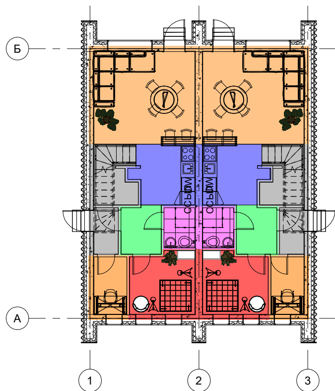
1 Zoning Scheme 1st level 1 : 100
