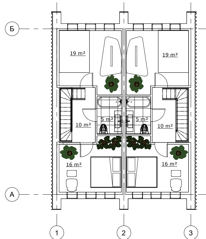
2 Areas 2nd level 1 : 100
