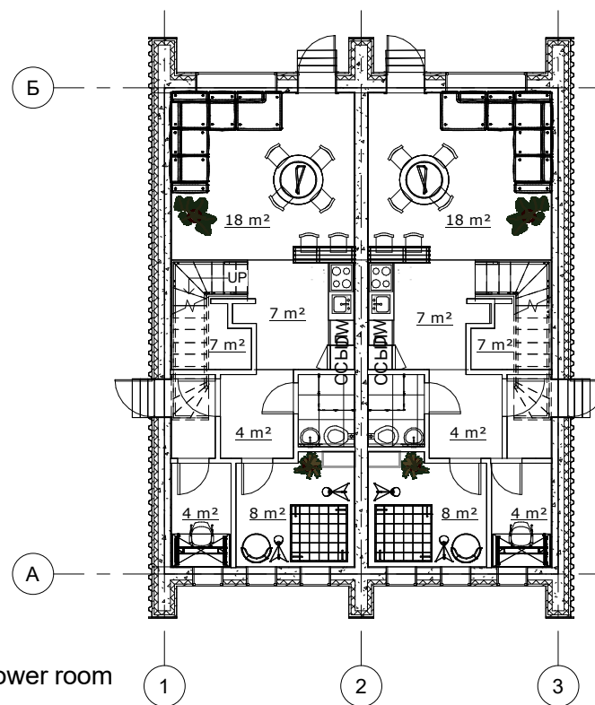
2 Areas 1st level 1 : 100
