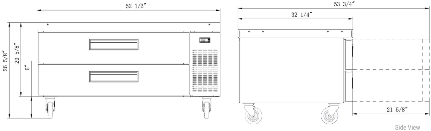
Side View
