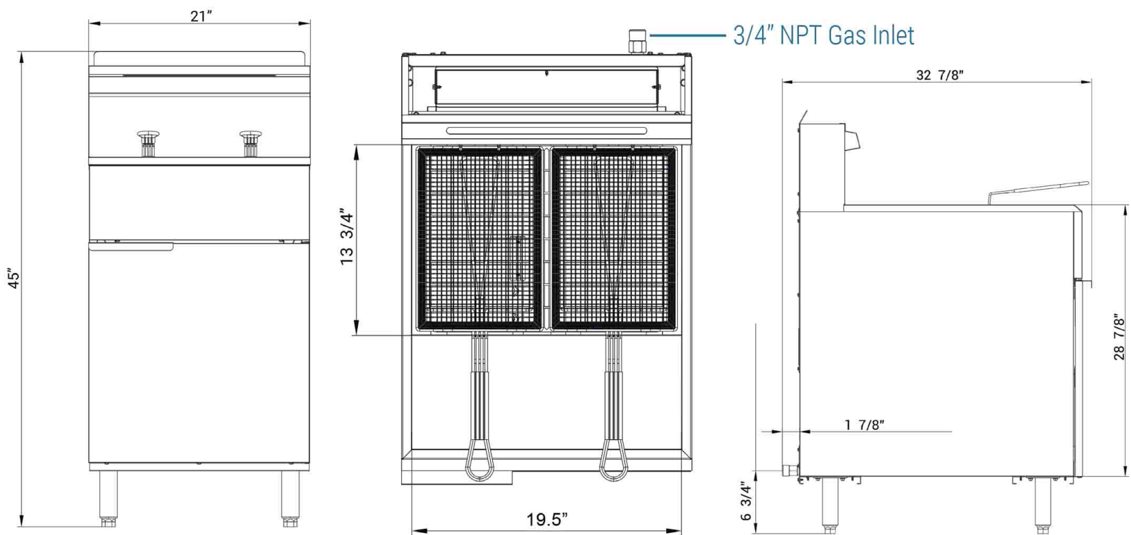
Front View
